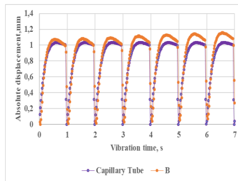
Fig. 7 Absolute displacements of B and tube (ID = 2.2 mm, f = 1 Hz, A = 1.03 mm)
