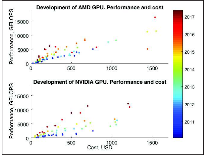
Fig. 2. AMD and NVIDIA models according to the release date.
