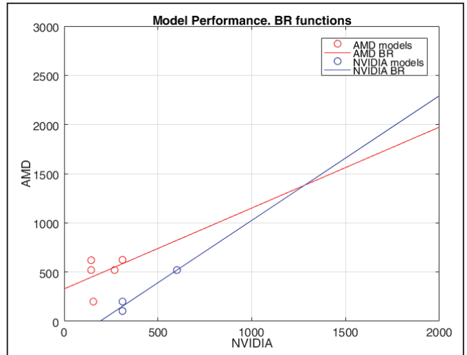
Fig. 5. Determination of NE for the chosen FOM based on BR functions
