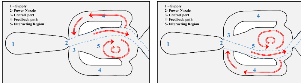
Figure 5 - Working principle of a sweeping jet actuator and visualization of internal flow (according to [15])
