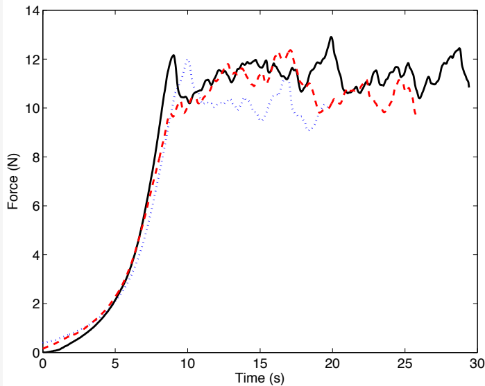
Fig. 3. Peel force with respect to time recorded during three tests.
