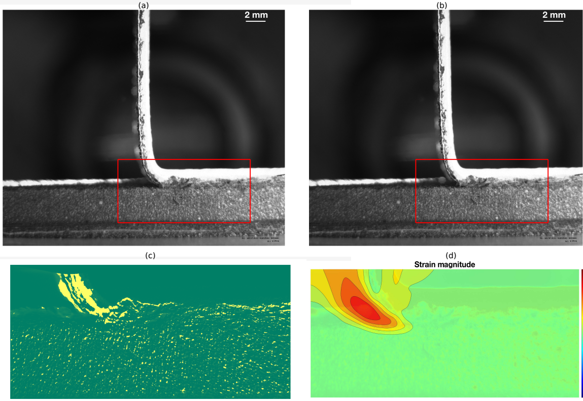
Fig. 4. Example of digital image correlation on large frame images: (a) reference image (b) deformed image, (c) gray level residual map after digital correlation, (d) resulting strain magnitude.
