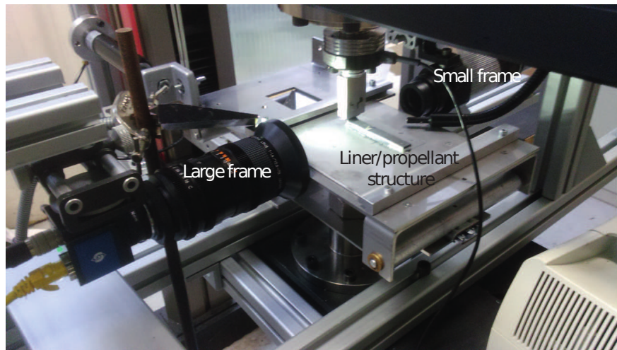
Fig. 1. Experimental setup.
