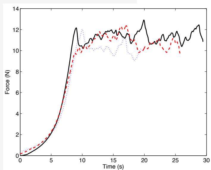
Fig. 3. Peel force with respect to time recorded during three tests.
