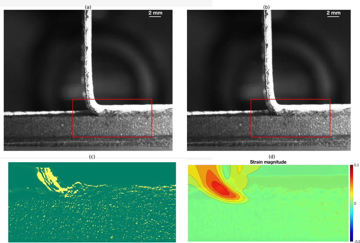
Fig. 4. Example of digital image correlation on large frame images: (a) reference image (b) deformed image, (c) gray level residual map after digital correlation, (d) resulting strain magnitude.
