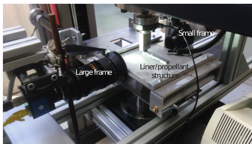
Fig. 1. Experimental setup.
