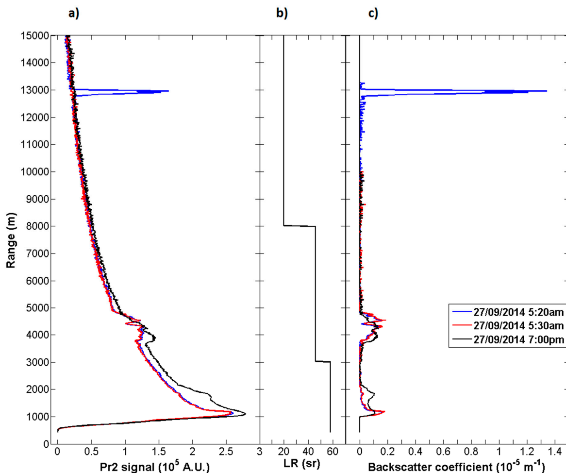
Figure 14. Lidar profiles obtained during the 27 September 2014 at 5:20 UT (blue), 5:30 UT (red) and 19:00 UT (black) presenting cirrus and forest fire aerosol layer respectively around 13 km and 4 km: (a) Pr 2 range corrected signal, (b) LIDAR Ratio and (c) backscatter coefficient.
