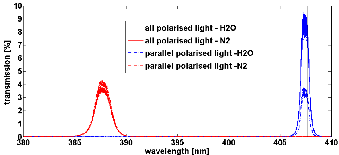
Figure 7. Transmission of the whole optical box for the Raman channels: nitrogen in red and water vapour in blue.
