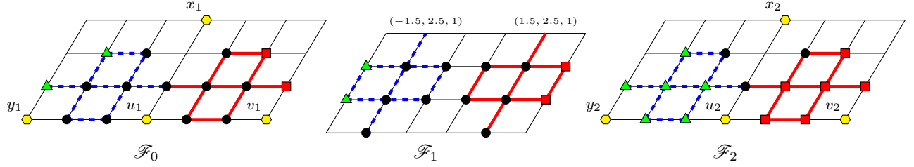
Figure 8: The vertices in B \cup B' \cup \{(-3, 1, 2), (0, 1, 2), (3, 1, 2)\} at distance at most 3 from u_1 (circles), v_2 (squares) or y_2 (triangles) and the vertices u_1, u_2, v_1, v_2, x_1, x_2, y_1 and y_2 (hexagons; thick lines: edges between vertices in B \cup \{(0, 1, 2), (3, 1, 2)\} ; dashed lines: edges between vertices in B' \cup \{(-3, 1, 2), (0, 1, 2)\} ).
