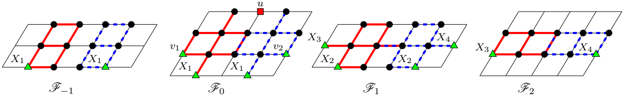
Figure 5: The vertex u (the square), the vertices in B \cup B' at distance at most 3 from u (circles) and the vertices at distance at least 4 from u in B \cup B' (triangles; thick lines: edges between vertices in B ; dashed lines: edges between vertices in B' ).
