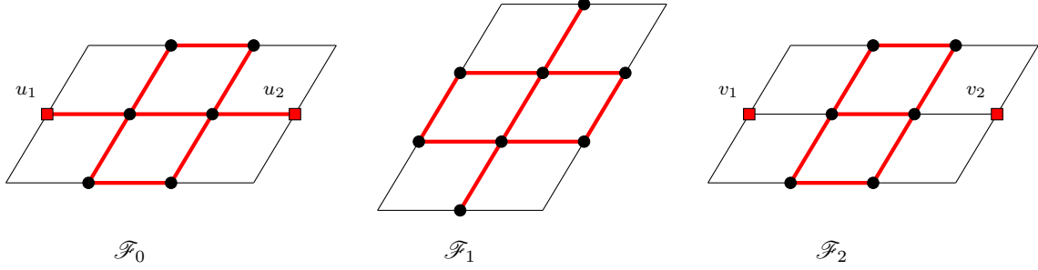
Figure 6: The vertices in B (circle) and the vertices u_1, u_2, v_1 and v_2 (squares; thick lines: edges between vertices in B ).
