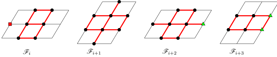
Figure 4: The vertex (i, j, k) (the square), the vertices in B at distance at most 3 from (i, j, k) (circles) and the vertices at distance at least 4 from (i, j, k) in B (triangles; thick lines: edges between vertices in B ).
