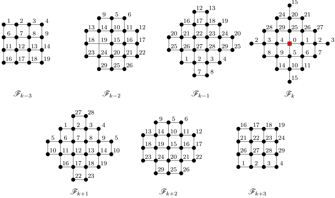
Figure 3: The colors of the vertices at distance at most 3 of a fixed vertex u of color 0 in the layer k of the graph \mathcal{F} (square: u ; circle: vertex at distance d of u , 1 \leq d \leq 3 ).
