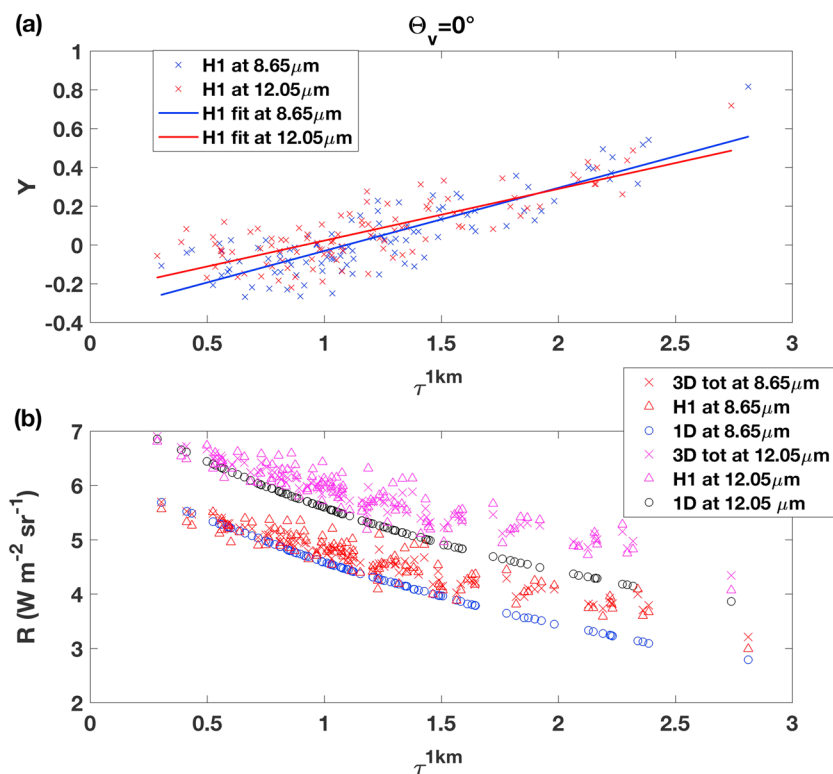
Figure 11. (a) Y values in (8) versus \tau^{1km} at 8.65 \mu\text{m} and 12.05 \mu\text{m} for the nadir view of cirrus 1; also shown is the a\tau + b adjustment term in (7), as determined by linear fit. (b) Three-dimensional total radiances, H1 hybrid model, and 1-D total radiance model.
