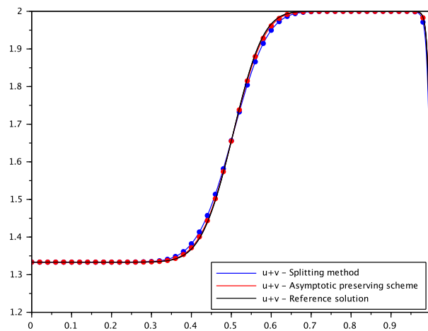
Figure 2: Comparison of the AP scheme and of the splitting method with a reference solution for several mesh sizes: 50 (up), 200 (center), 800 (bottom) — u + v vs. space.
