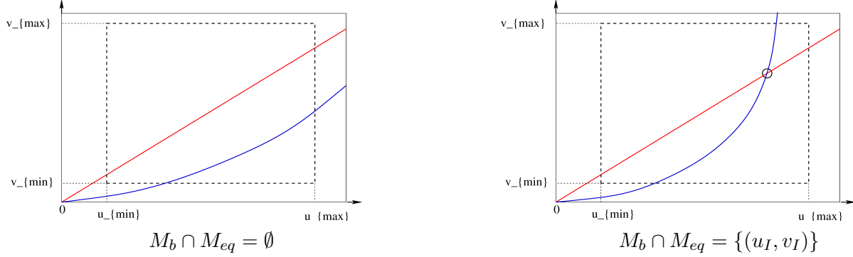
Figure 1: Plot of the two equilibrium manifolds. Either M_{eq} (blue) intersects M_b (red) inside [u_{min}, u_{max}] \times [v_{min}, v_{max}] (right), either it does not (left).
