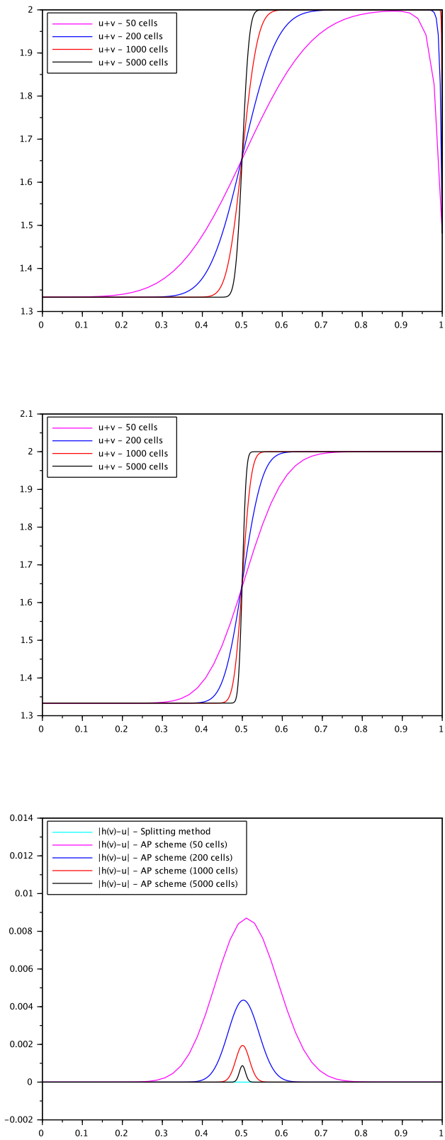
Figure 4: Results provided by the splitting method (left: u + v ) and by AP scheme (center: u + v , right: |h(v) - u| ), for several mesh sizes: 50, 200, 1000, 5000 cells.
