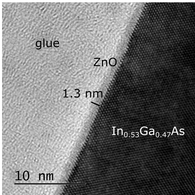
Figure 4: TEM cross-sectional image of a ZnO layer on In 0.53 Ga 0.47 As obtained after 25 ALD cycles ( T_{\text{substrate}} = 120^{\circ}\text{C} ).
