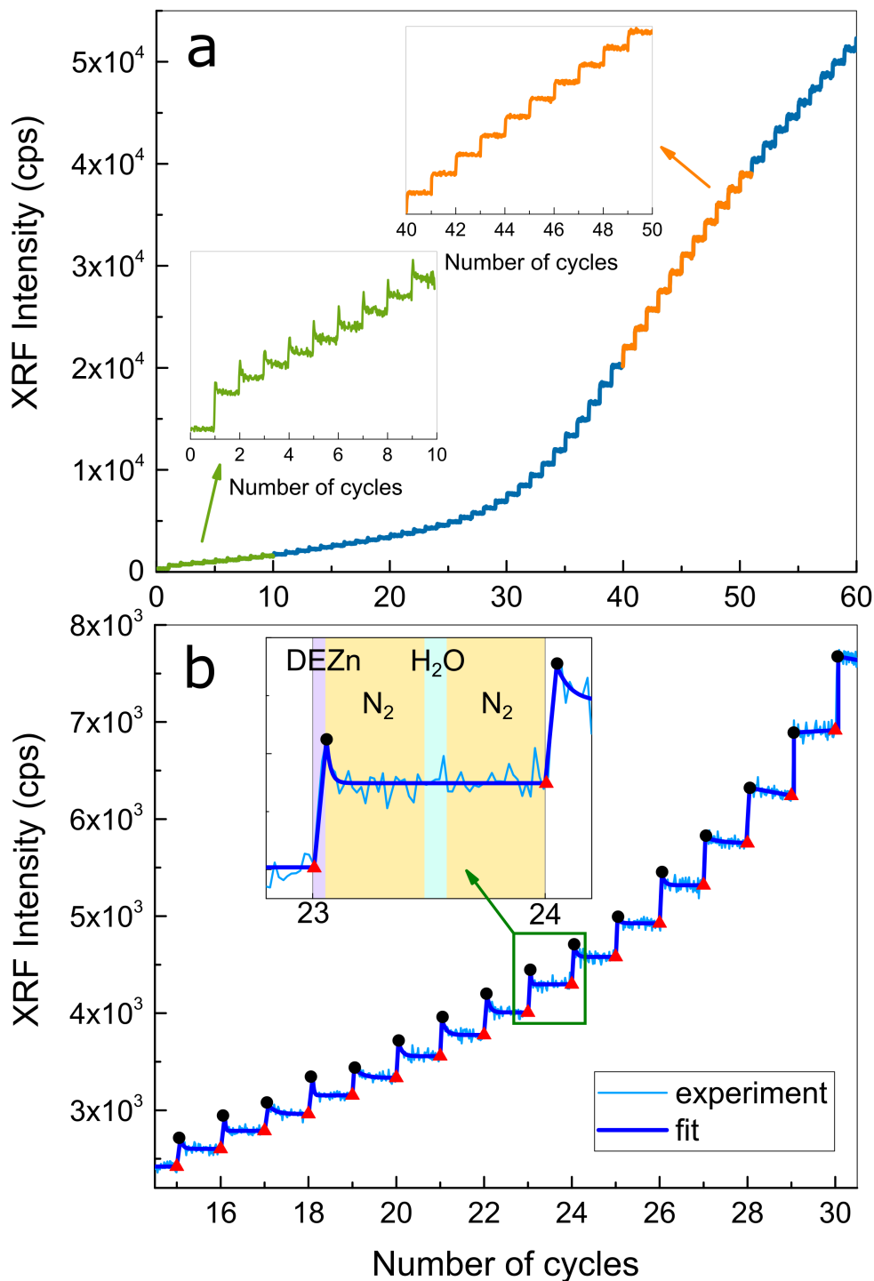
Figure 2: (a) Zn K_{\alpha} X-ray fluorescence intensity ( T_{substrate} = 120^{\circ}\text{C} ) vs. cycle number. The insets show the Zn fluorescence intensity (green curve) at the early stages, as compared with intensity at the later stages (orange curve). (b) The experimental Zn fluorescence intensity (light blue curve) and fit (dark blue curve) for cycles 15-30. The inset shows the fluorescence intensity and fit curve for cycle 24. Black closed circles indicate the Zn fluorescence intensity at the end of the DEZn pulse, and red closed triangles indicate the Zn fluorescence intensity at the end of each ALD cycle.
