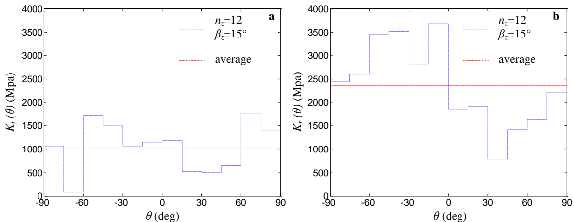
Figure 6. Evolution of the specific cutting coefficients (a) K_t(\theta) and (b) K_r(\theta) identified through a piecewise constant model
