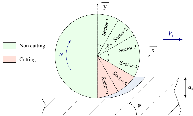
Figure 5. Piecewise constant model
