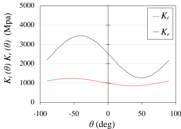
Figure 7. Analytical model of the specific cutting coefficients in relation to fibre orientation, (a) K_t(\theta) and (b) K_r(\theta) , identified from the experiments.
