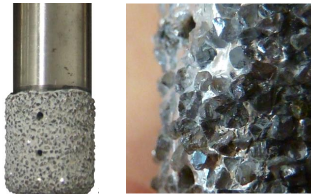
Figure 1. Diamond abrasive cutter with grits size of 852\ \mu\text{m}
