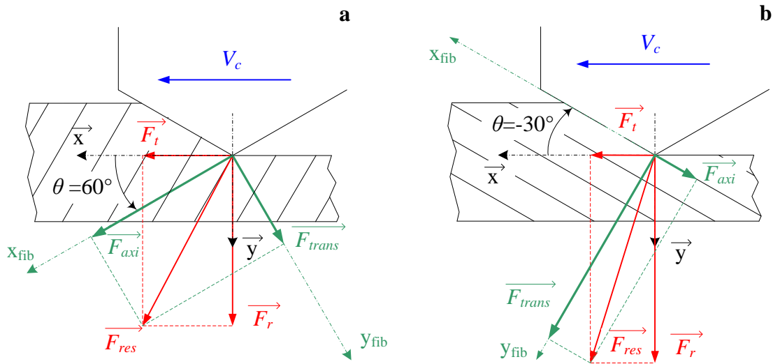
Figure 10. Cutting forces projection onto fibres reference system
