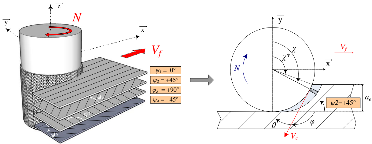
Figure 4. Example of configuration of a multidirectional laminate, composed of m=4 plies with unidirectional fibres.
