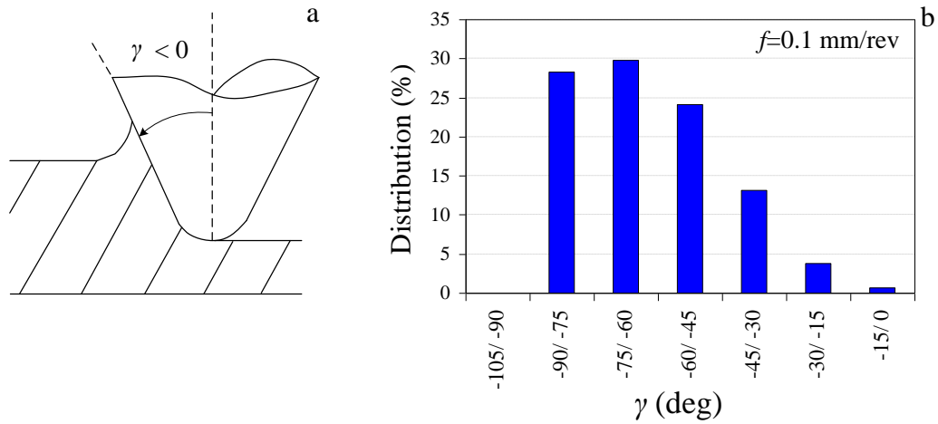
Figure 9. (a) Definition of grits rake angle, (b) Distribution of grits rake angle on a diamond abrasive cutter (grits size of 852 \mu\text{m} ).
