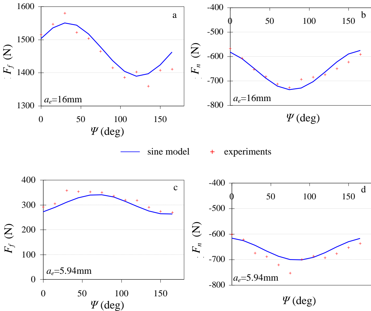
Figure 8. Experimental and simulated feed forces F_f (a-c) and normal forces F_n (b-d), a_e = 16\text{ mm} (a-b) and a_e = 5.94\text{ mm} (c-d)
