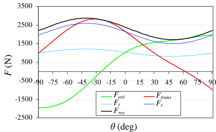
Figure 11. Cutting forces in orthogonal cutting configuration
