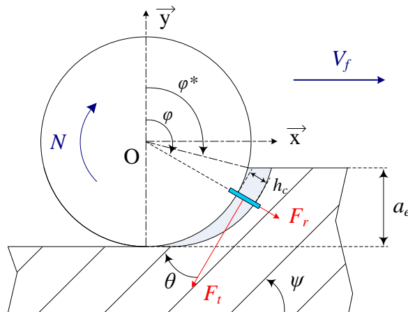
Figure 2. Cutting forces at the cutting edge
