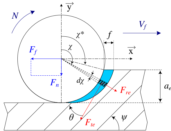
Figure 3. Elementary cutting forces applied on a d\chi sector
