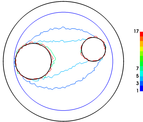
FIGURE 4. Validation of the level set method ( T = 25 )
