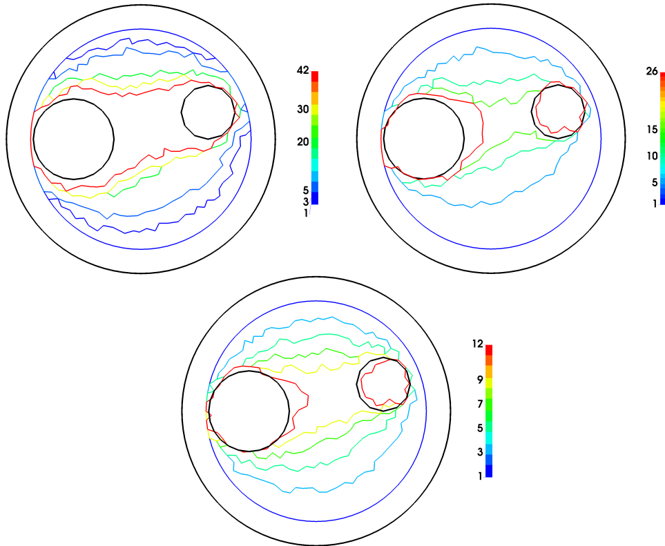
FIGURE 5. Two discs and exact data. Top left: T = 10 . Top right: T = 15 . Bottom: T = 25
