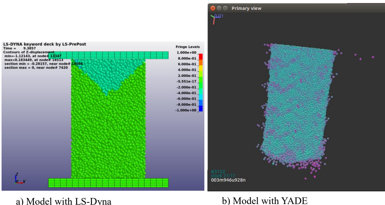
Figure 1 Examples of DEM models used for uniaxial compression of plain concrete
