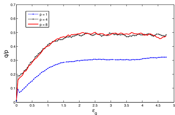
Figure 2 Shear loading for 3 different values of the confining dimensionless pressure ( p=1,4,8 ).
