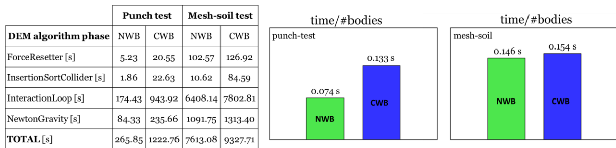
Figure 2 Comparison of the computational time for the different approaches (NWB and CWB) in the two test conditions.
