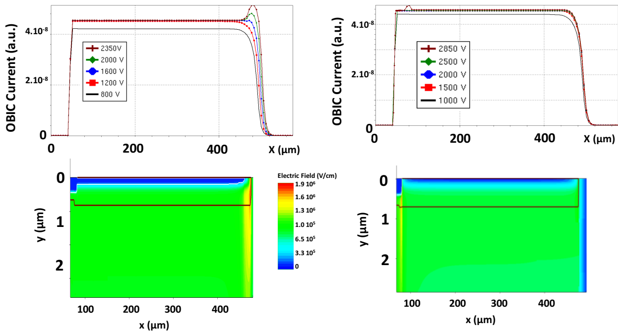
Fig. 5. Simulation results of OBIC current for both structures (device #1 from 800 V up to 2350 V and device #2 from 1000 up to 2850 V) and the corresponding electric field distribution at near breakdown voltage for both cases.
