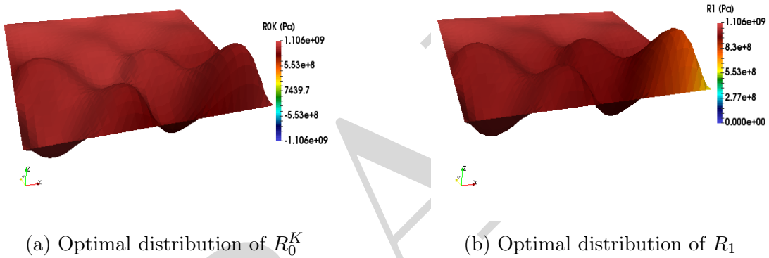
Figure 21: Example three, shape and anisotropy optimization: optimal distribution of the anisotropy polar parameters.
