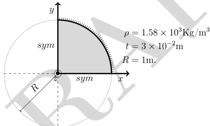
Figure 4: Circular plate geometry and boundary conditions.
