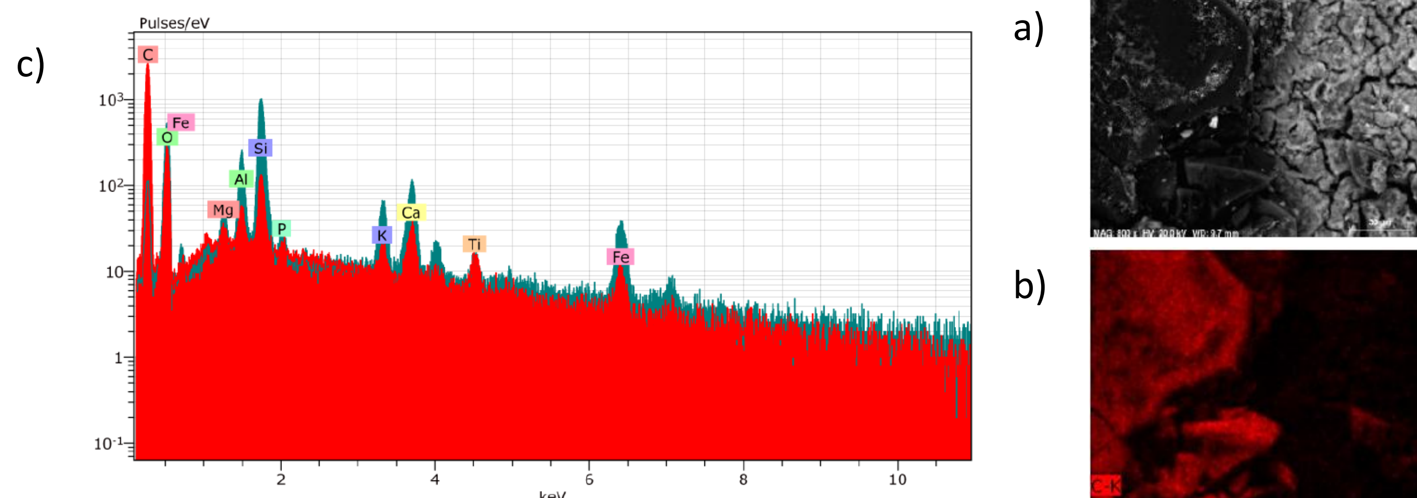
Fig. 3 - (a) Surface observation obtained by SEM. (b) C-K \alpha elemental mapping obtained by EDS. (c) Comparison of EDS spectra revealing the presence of a higher amount of carbon on the darkest region of the sherd.
