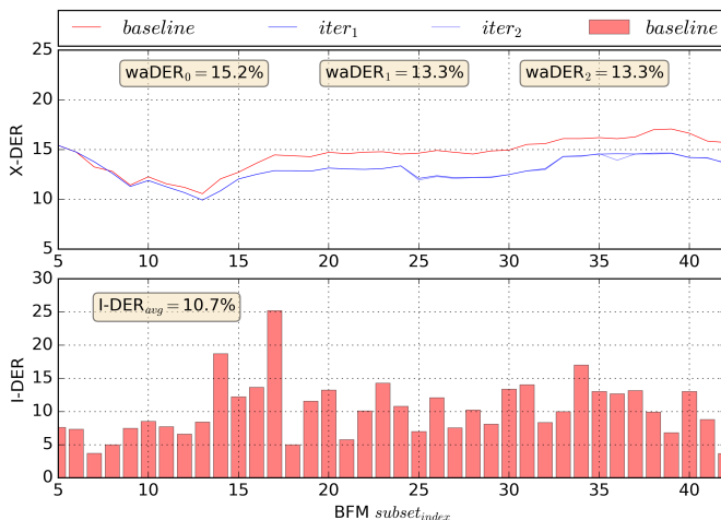
Figure 6. Cross-recording DER of the BFM corpus subsets, for iteration 0 to 2, using PLDA for scoring and adaptation. Experiment parameters are ( \lambda_I = 10, \lambda_X = 10, \alpha = 0.5 ).
