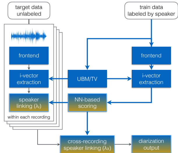
Figure 1: Overview of the diarization framework.
