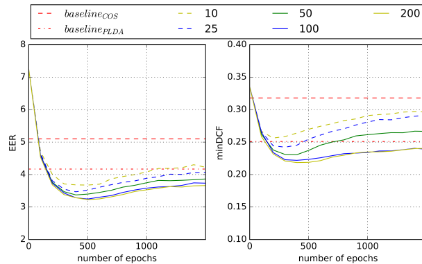
Figure 3: Average EER and minDCF on the two target datasets, using different number of nearest neighbors for training. Each condition is repeated 20 times and averaged.
