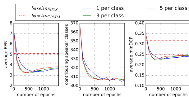
Figure 4: Influence of the number of examples provided per class. Average EER, minDCF and number of speaker classes contributing to the loss, on the two target datasets.
