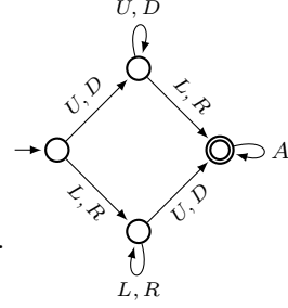
Figure 7: The automaton \mathcal{A}_\pi when \pi = 1 .
