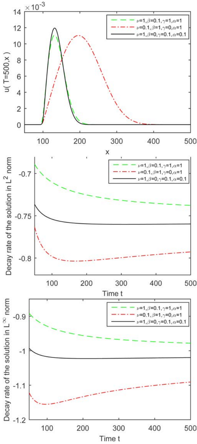
FIGURE 4 Numerical solutions and the ratios R_2 and R_\infty using the Gear scheme when \nu = 1 ou 0.1 and \Delta t = 0.1 [Color figure can be viewed at wileyonlinelibrary.com ]
