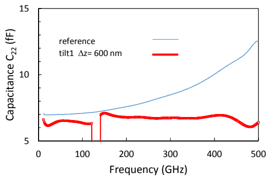
Fig. 9: Capacitance “C22” versus frequency of the transistor-open obtained from EM simulation including a TRL calibration with an ideal probe and with tilt default (reference: \Delta z=0\text{nm} , tilt1: \Delta z=600\text{nm} ).
