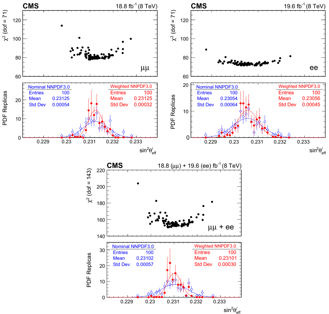
Fig. 6 The upper panel in each figure shows a scatter plot in \chi^2_{\text{min}} vs. the best-fit \sin^2 \theta_{\text{eff}}^{\ell} , for 100 NNPDF replicas in the muon channel (upper left), electron channel (upper right), and their combination (below). The
