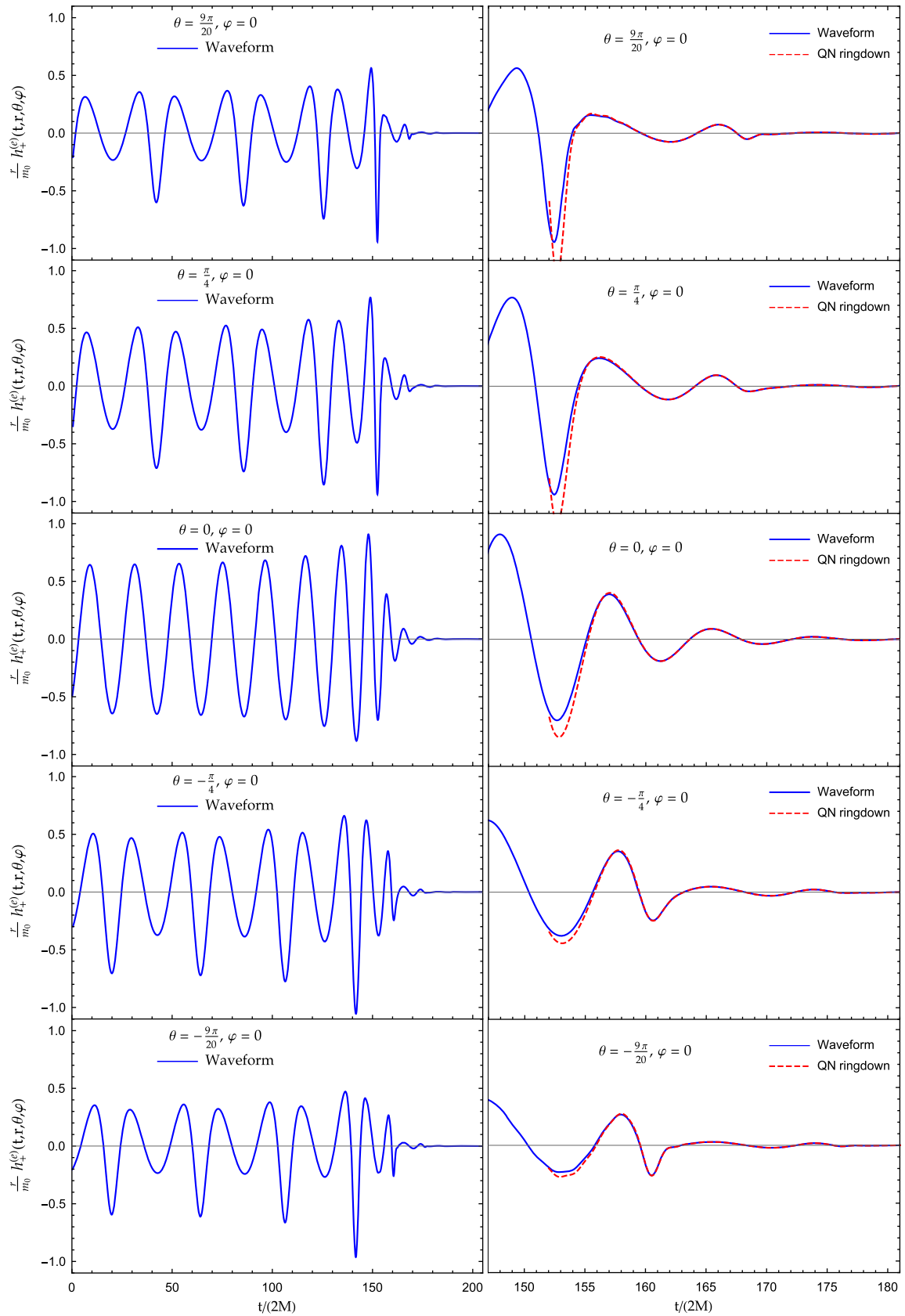
FIG. 4. Multipolar gravitational waveforms h_+^{(e)} observed at infinity for various directions above the orbital plane of the plunging particle. We consider \varphi = 0 and we study the distortion of the multipolar waveform and of the associated quasinormal ringdown when \theta varies between -\pi/2 and +\pi/2 . We note that, for \theta = 0 , only the (\ell = 2, m = \pm 2) modes contribute to the signal.
