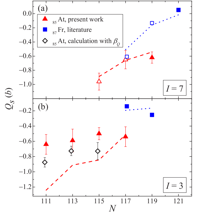
FIG. 12. Comparison of Q_S^{\text{add}} and Q_S^{\text{exp}} for isotopes of astatine (red triangles) and francium (blue squares) with (a) I = 7 ( \pi h_{9/2} \otimes \nu f_{5/2} ) and (b) I = 3 ( \pi h_{9/2} \otimes \nu p_{3/2} ). The filled symbols indicate ground states and the hollow ones indicate isomeric states. Results of the calculations using the quadrupole additivity rule [Eq. (15)] are indicated by the red-dashed and blue-dotted lines for the astatine and francium isotopes, respectively. The black diamonds in panel (b) represent calculations made using Eq. (14), with \beta_Q taken from the Q_S value of the adjacent even- N At.
