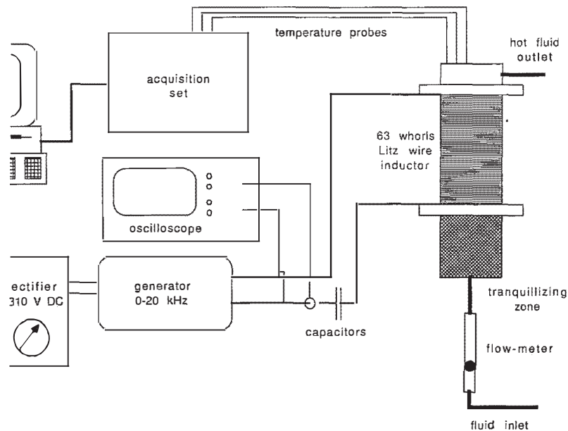
FIG. 2. Experimental apparatus.
