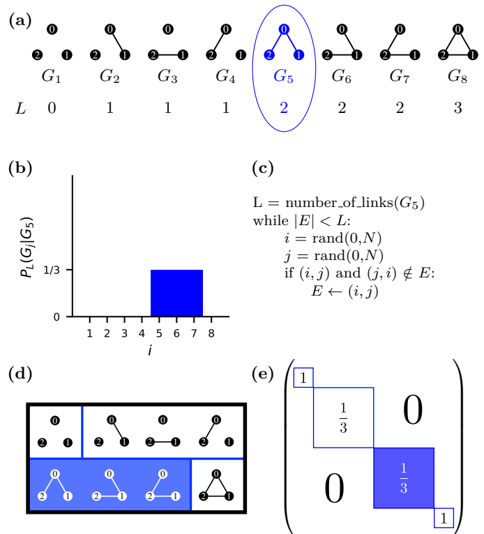
FIG. II.4: Equivalent MRRM representations. We consider the state space of all simple graphs with three nodes and the MRRM \mathbf{P}[L] which constrains the number of edges L in a graph. The state space \mathcal{G} contains eight states (graphs) and is ordered as shown in (a). The input network is taken to be G^* = G_5 (highlighted in blue) for which L^* = L(G_5) = 2 . Panels (b)-(e) illustrate graphically the four equivalent representations of \mathbf{P}[L] when applied to G_5 : (b) The conditional probability P_L(G_j|G_5) gives the probability to generate each state G_j using \mathbf{P}[L] with G_5 as the input state. (c) A shuffling method corresponding to \mathbf{P}[L] samples graphs G_j from the subset of networks with L(G_5) = 2 links, \mathcal{G}_{L(G_5)} \subset \mathcal{G} according to P_L(G_j|G_5) . (d) The partition of \mathcal{G} induced by \mathbf{P}[L] consists of the four distinct sets: \mathcal{G}_0 = \{G_1\} , \mathcal{G}_1 = \{G_2, G_3, G_4\} , \mathcal{G}_2 = \{G_5, G_6, G_7\} (marked in blue), and \mathcal{G}_3 = \{G_8\} . (e) The block-diagonal stochastic matrix \mathbf{P}^L gives the probability to generate any output state G_j from any given input state G_i (the block corresponding to the input state G^* = G_5 is marked in blue).
