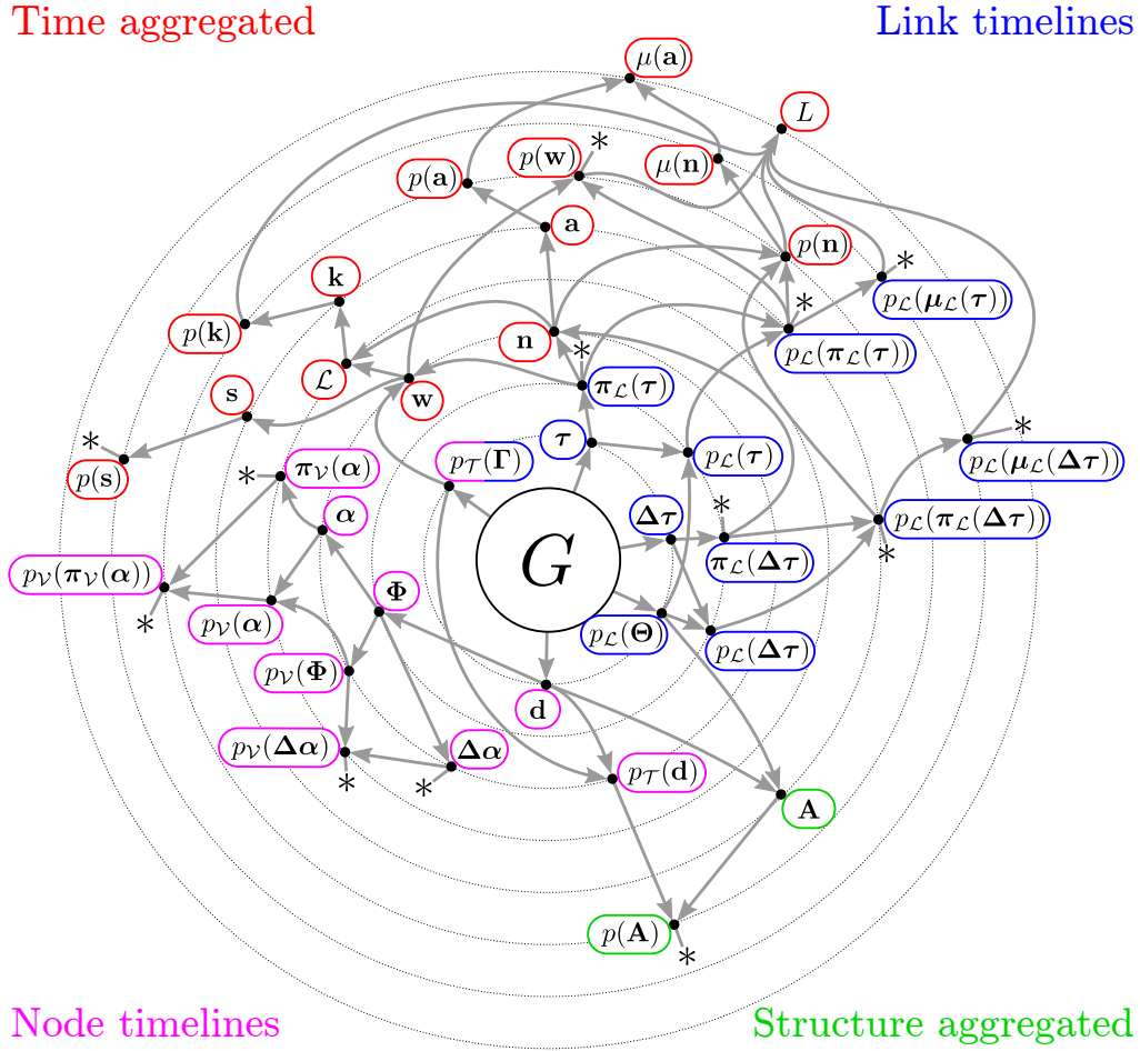
FIG. 7: Feature hierarchy diagram. An arrow from a higher ranking (more central) to a lower ranking feature (node in the diagram) indicates that the former feature is finer than the latter. Thus, a MRRM that constrains the feature in a given node also constrains all features of downstream nodes. Conversely, a MRRM that randomizes (i.e. does not constrain) the feature of a given node does not constrain any of the features of upstream nodes either. See Tables I and II for definitions of the features. A star (*) emanating from a node indicates that lower hierarchical levels follow as shown in Fig. 6. The color coding shows what type of characteristics the features correspond to: time-aggregated characteristics (i.e. topological and weighted), link-timeline characteristics, node-timeline characteristics, and structure-aggregated characteristics (i.e. purely temporal).
