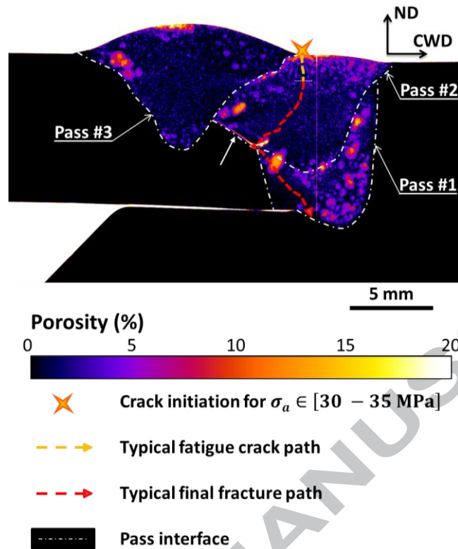
Fig. 8: Representation of the porosity distribution of a GMAW assembly in the CWD-ND plane obtained by X-ray microtomography analyses. The evolution of the porosity from pass to pass and location of large pores in the periphery of passes was evidenced. A continuous defect region highlighted with a white arrow was found in the mid-section of the joint assembly at the interface of pass #2/HAZ. The crack path of a fatigue-tested specimen in the high stress amplitude regime obtained via confocal microscopy was reported on the porosity distribution (green dashed line). The crack initiated at the interface of pass #2/pass #3 at the top surface of the specimen.
