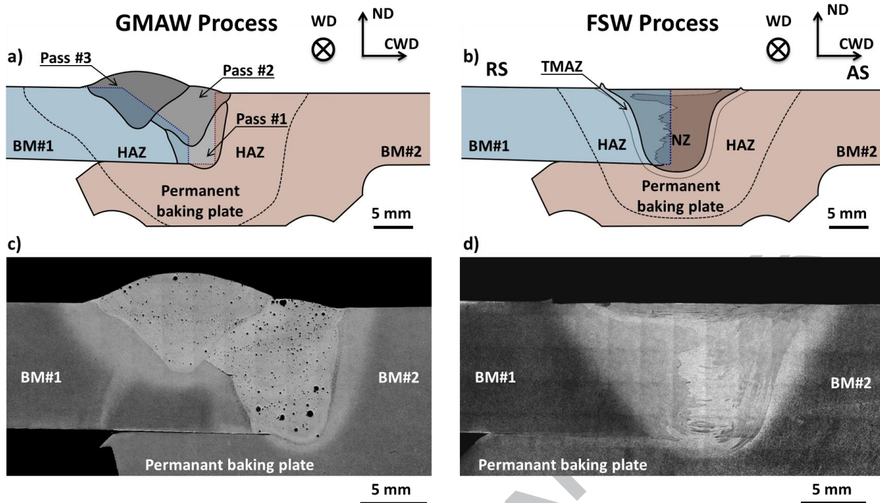
Fig. 1: Cross-section view of the GMAW process and FSW process configurations: Schematic illustrations of the design of the structural components a) prior to GMAW welding, where the three welding passes were superimposed and the heat-affected zone (HAZ) was shown and, b) prior to FSW welding, where a mixing area after welding was superimposed and the nugget zone (NZ), the thermo-mechanically affected zone (TMAZ) and the heat-affected zone (HAZ) were shown, and c) macrograph showing the different passes of the weld and the HAZ in a neighboring area of the weld. Micrometer- and millimeter-size pores (black dots) were found within the three passes of the weld. Millimeter-size pores were particularly found within passes #1 and #2; d) macrograph showing the delimitation of the interface of NZ/TMAZ and the mixing of the two original structural components within the NZ.
