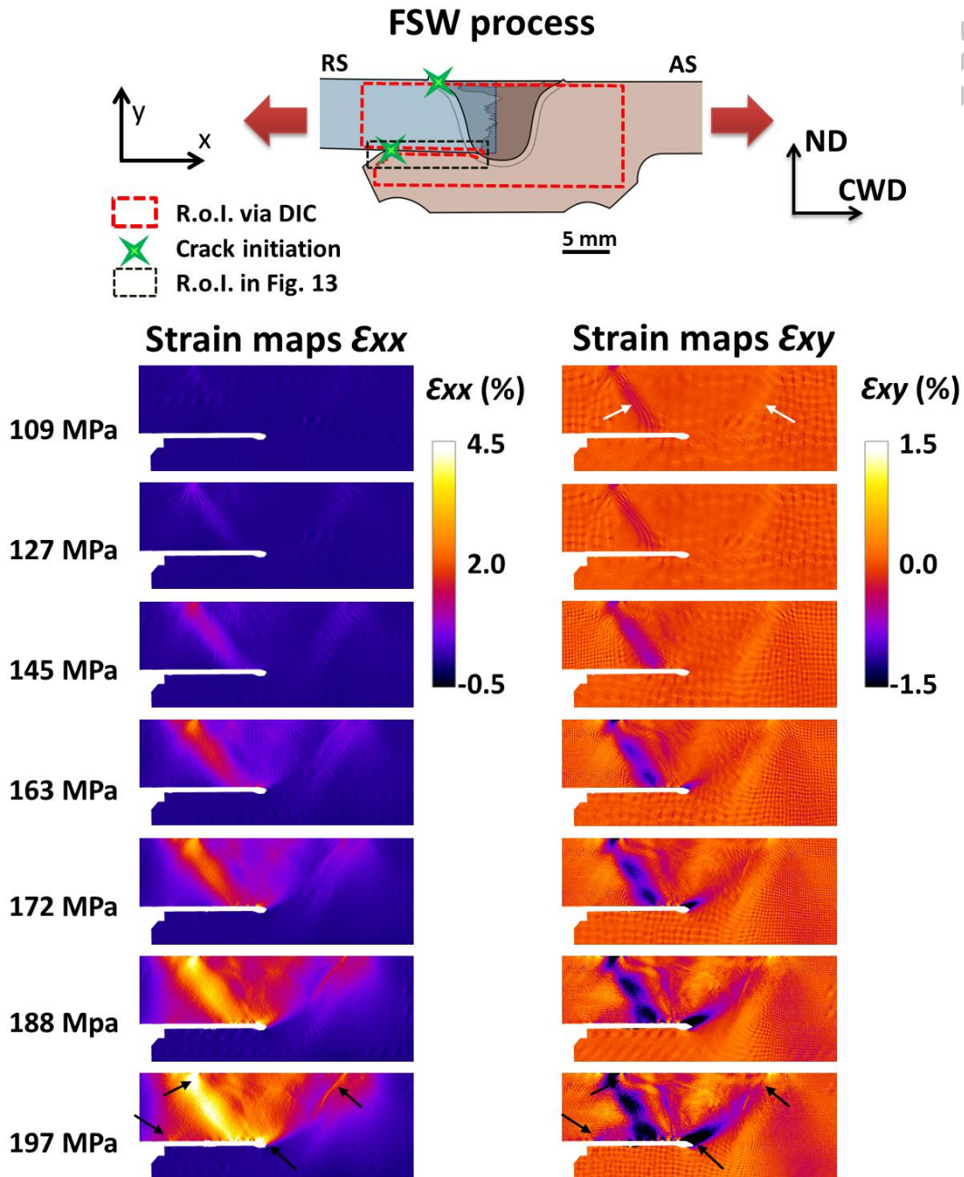
Fig. 12: Schematic illustration of the region of interest for DIC experiments performed on the FSJ configuration and strain maps ( \epsilon_{xx} and \epsilon_{xy} ) for different loading conditions. Strain localization occurred in the HAZ on both sides of the
