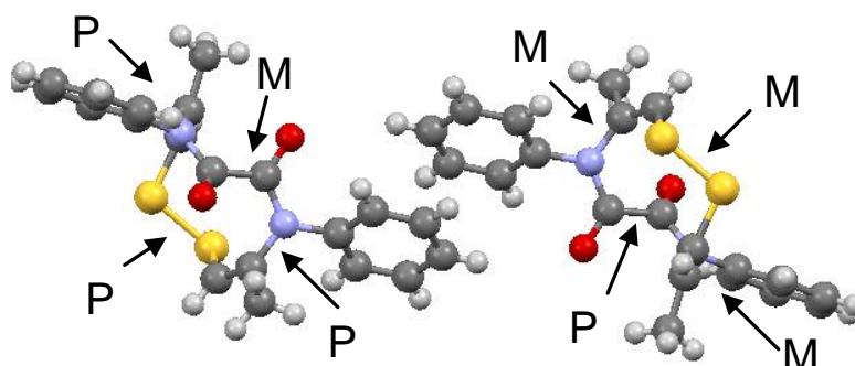
Figure 3. X-ray crystal structure of 3 : for sake of clarity only two enantiomers among the four pairs of enantiomers found in the cell are displayed. The M or P configuration of each axis is given.
