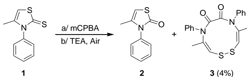
Scheme 1. Oxidation of thiazoline-2-thione 1 yielding thiazolinone 2 and unknown 3 as a very minor compound
