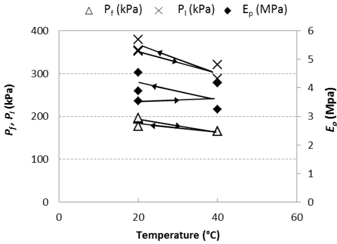
Figure 8 : Impact of temperature variation on pressuremeter test parameters in illitic compacted soil.
