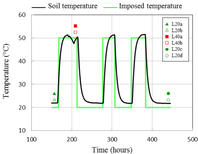
Figure 9: Temperature variation in the loam at 150 mm from the edge of the container and the chronology of the tests: 3 heating-cooling cycles (20-50-20 °C) and time of the pressuremeter tests.
