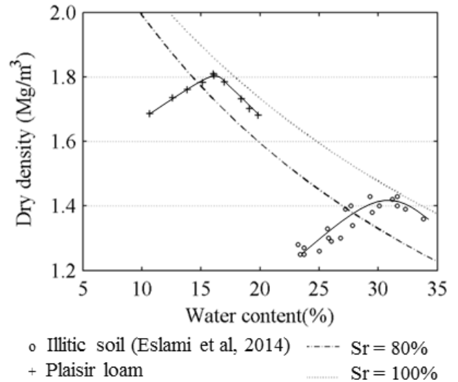
Figure 2: Compaction curves of the studied materials.
