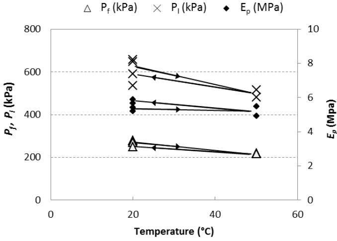
Figure 11 Impact of temperature variation on pressuremeter test parameters in compacted loam.
