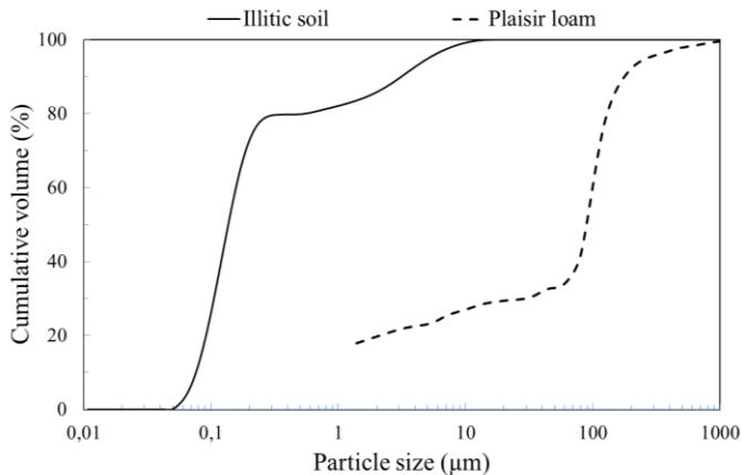
Figure 1. Granulometric curves of the studied materials.
