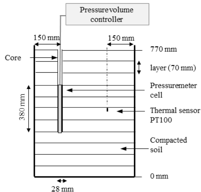
Figure 4: Position of the pressuremeter cell.
