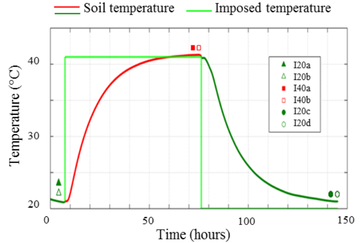
Figure 6: Temperature variation in the illitic compacted soil at 150 mm from the edge of the container and the chronology of the tests: heating-cooling cycle (20-40-20 °C), time of the pressuremeter tests (I20a, b, c, d, I40a, b).
