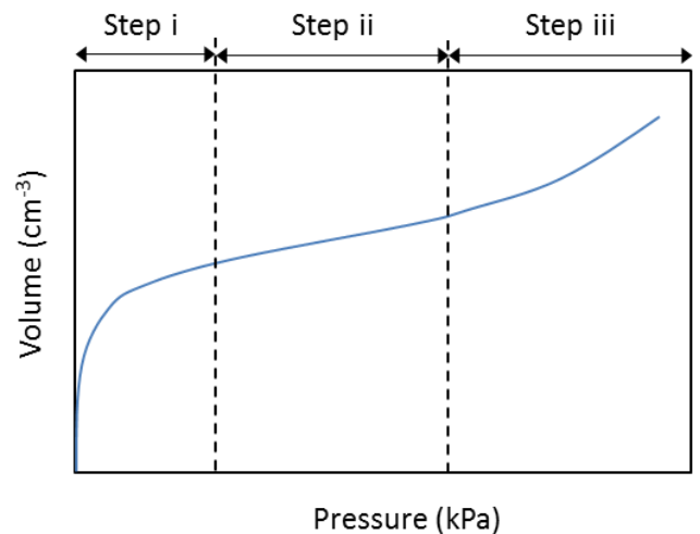
Figure 5 : The 3 steps of a pressuremeter curve
