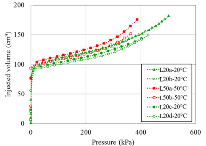
Figure 10: Pressuremeter heating curves for the tests on loam material: heating-cooling cycle (20-50 °C).
