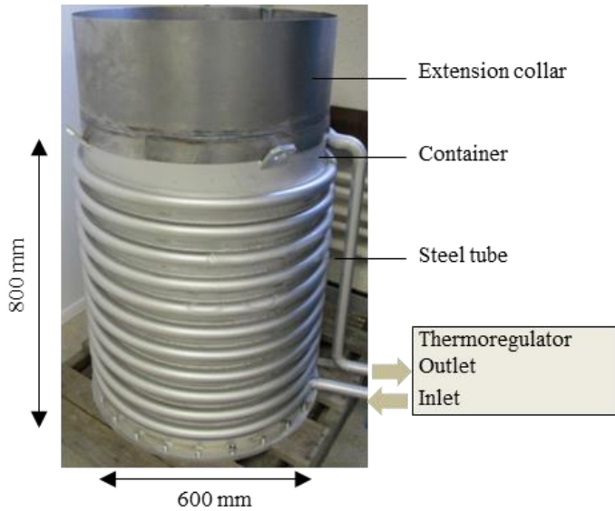
Figure 3: Thermo-regulated metric scale container.
