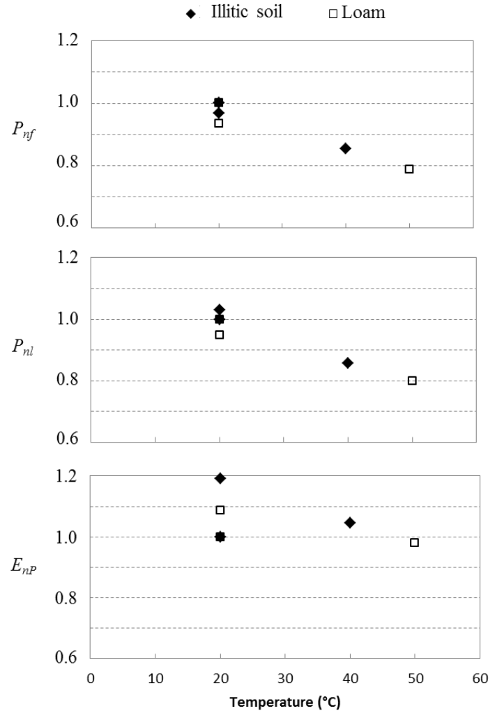
Figure 12: Evolution of the normalized parameters according to the test temperature for two materials.
