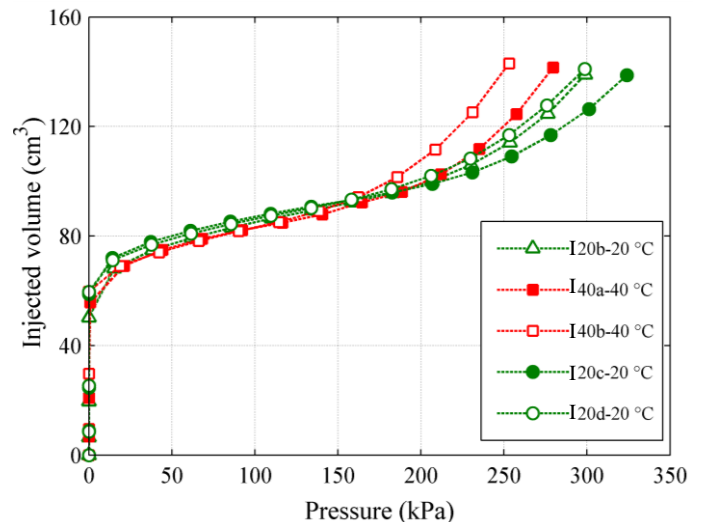
Figure 7: Pressuremeter curves for the tests on illitic material: I20b, I40a-b and I20c-d.
