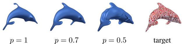
Figure 11. Registered ellipsoid onto a dolphin with missing triangles as in Figure 9. The true proportion of triangles of the target is p^* = 0.6 . When p > p^* (resp. p < p^* ) the resulting matching looks thinner (resp. bulgy) due to the difference in total area.
