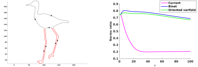
Figure 2. Behavior of the different metrics. On left, a shape with thin elongated components in red. On right, a plot of the ratios between the norm of the red part with the norm of the entire shape for increasing scales \sigma for the Gaussian function \rho . Note the rapid decrease in the case of currents, due to the cancellation of oppositely oriented pieces ‘close’ to each other with respect to \sigma .
