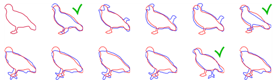
Figure 3. Least accurate top 12 retrieval of a query shape.
