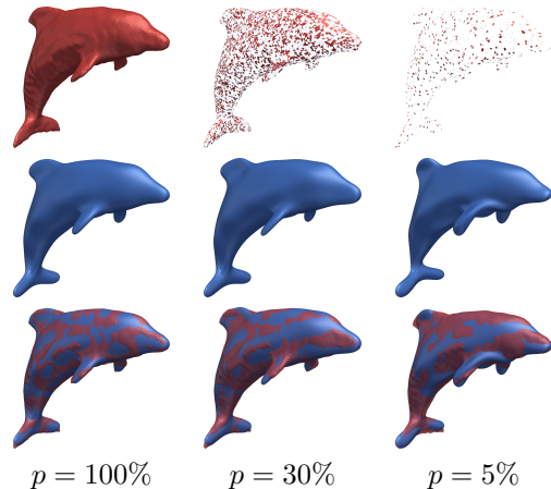
Figure 10. Three registrations onto a target with various ratios of missing faces. The proportion (1 - p) of missing triangles is known. Corresponding target shapes are on the first row. Deformed ellipsoids are plotted on the second row. Comparison between the deformed ellipsoid and the complete target are shown on the third row.
