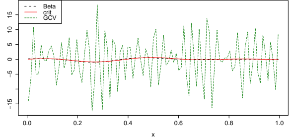
Figure 3: Left: comparison of estimators \hat{\beta}_m when m is selected by minimization of the penalized criterion \text{crit} defined by (5) or the CV criterion. Right: comparison with the GCV criterion. n = 2000 , \lambda_j = j^{-3} .
