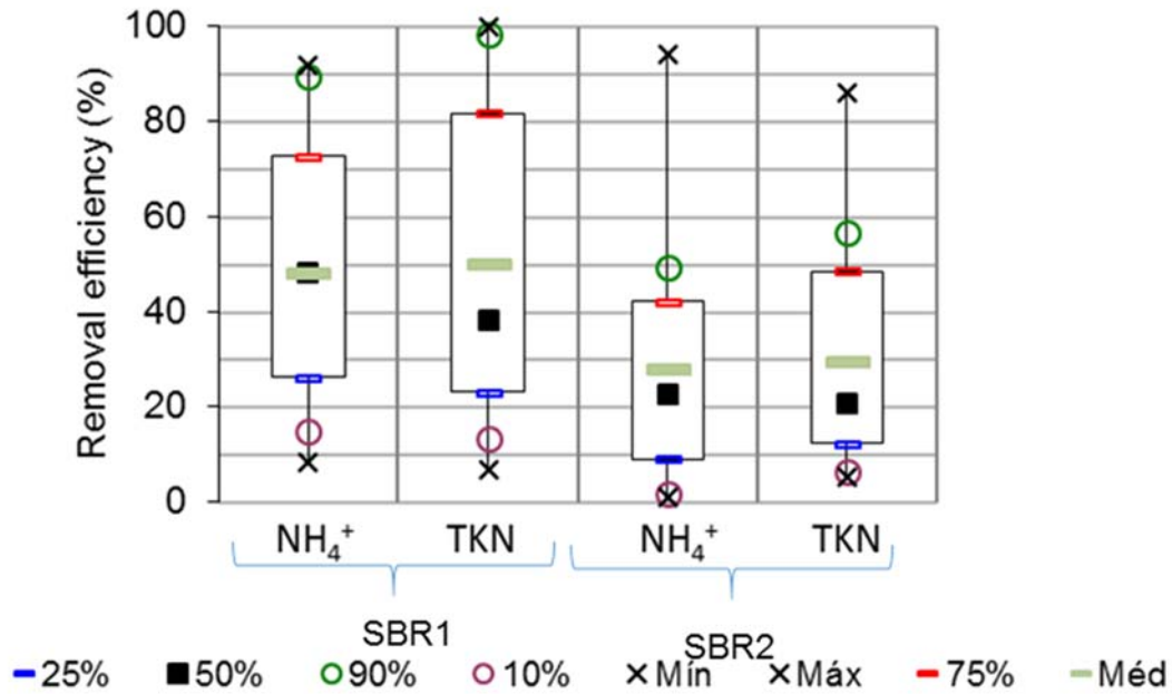
FIGURA 9. Boxplot: Removal efficiency of \text{NH}_4^+ and TKN - SBR1 and SBR2
