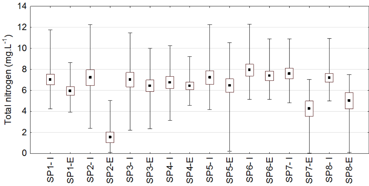
FIGURE 5. Nitrogen concentrations for influent (I) and effluent (E)
