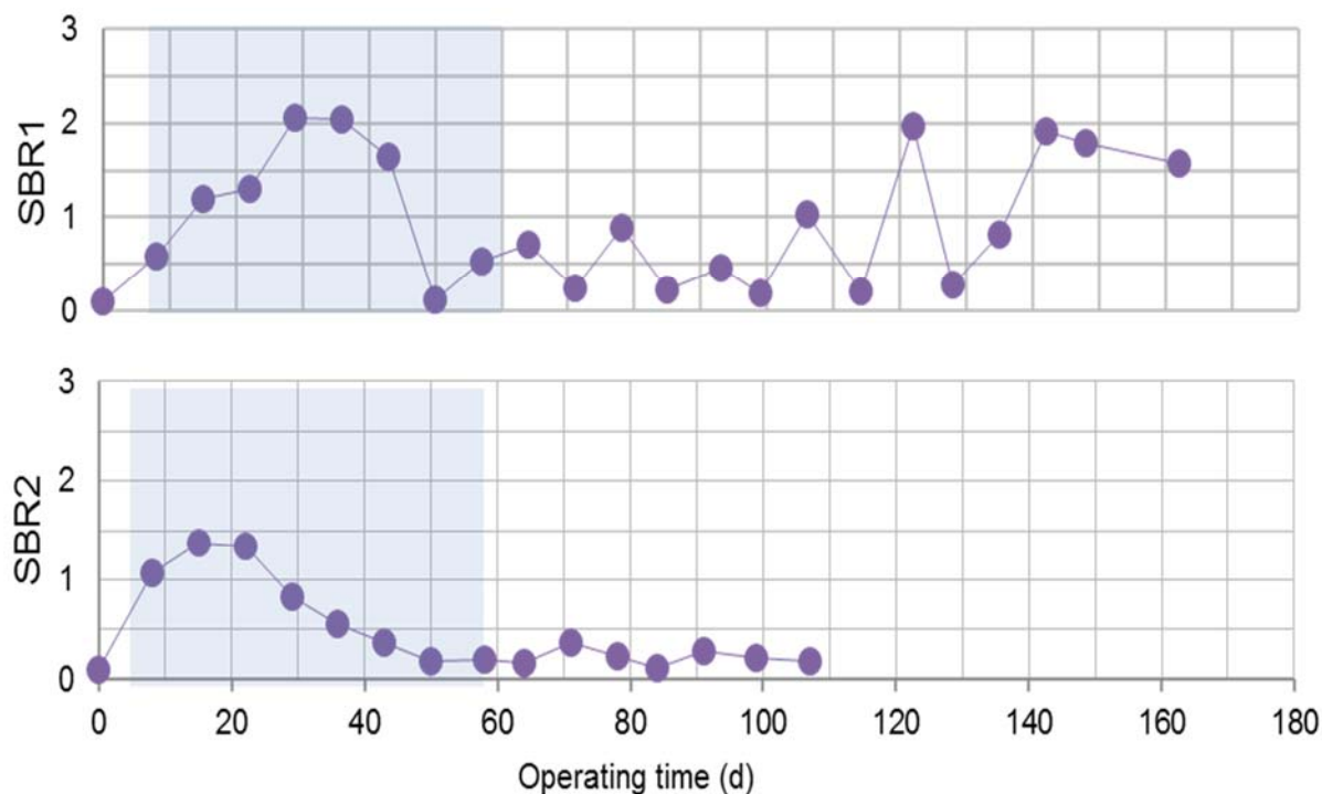
FIGURE 3. MLVSS (g.L -1 )
