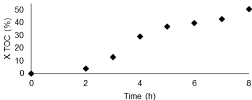
FIGURE 1. TOC conversion (%) for pH (initial) = 5 and R = 7.8
