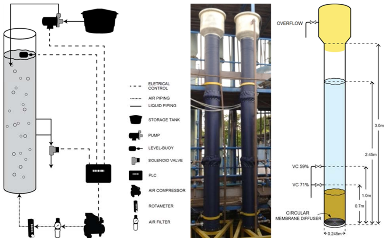
FIGURE 2. Experimental scheme (left); Photograph of reactors (center), Graphic diagram (right).
