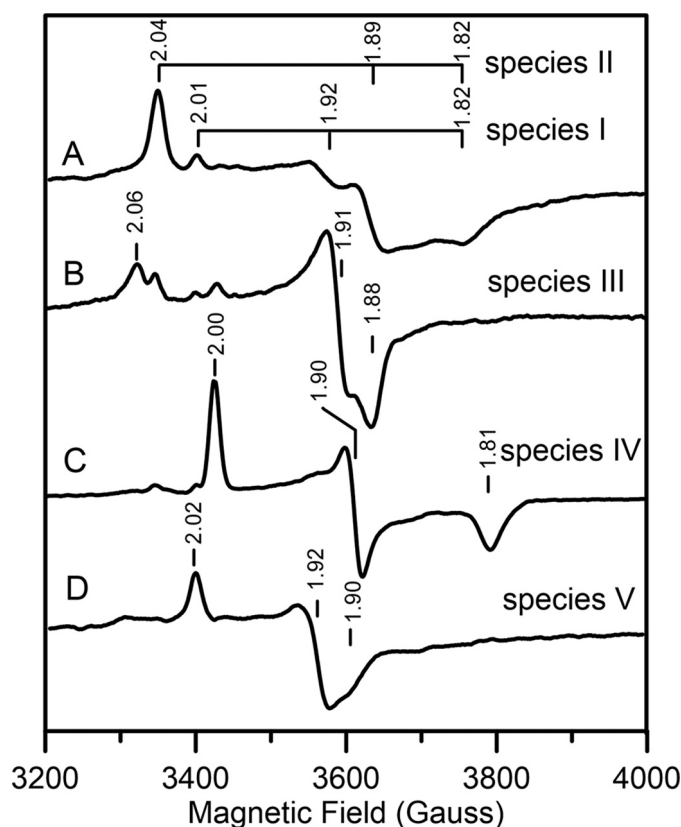
Figure 3. X-band EPR spectra of reduced [ \text{Fe}_2\text{S}_2 ] ^{1+} center in AtDHAD. All spectra presented were recorded at 35 K using 9.60 GHz microwave frequency, 6.4 G modulation amplitude, and a microwave power of 5 mW, except that B used 1 mW microwave power. A, dithionite-reduced DHAD; B, dithionite-reduced DHAD frozen immediately after addition of substrate; C, sample (B) after incubation with substrate at room temperature for 30 min; D, dithionite-reduced DHAD after incubating with DTT. The principal g-values corresponding to the major component(s) in each spectrum are indicated.
