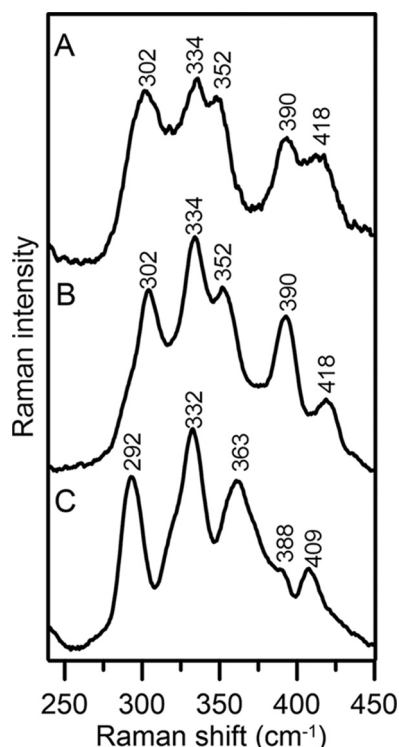
Figure 4. Low temperature (17 K) resonance Raman spectra of as-purified AtDHAD using 488-nm laser excitation line. A, as-purified DHAD; B, as-purified DHAD after addition of substrate; C, as-purified DHAD incubated with DTT. Bands resulting from the frozen buffer solution have been subtracted from all spectra.
