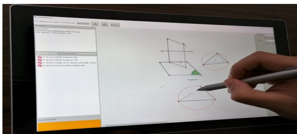
Fig. 17: Prototype interface
