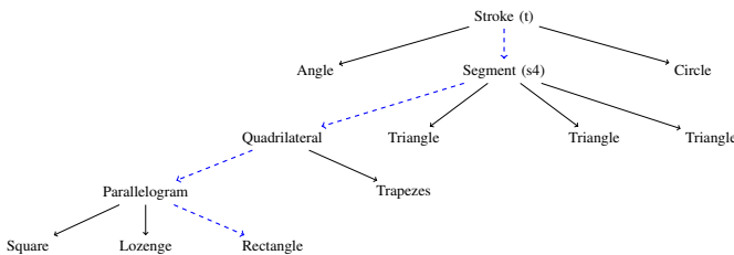
Fig. 6: Analysis tree
