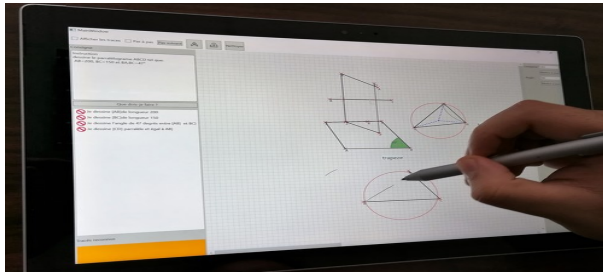
Fig. 17: Prototype interface
