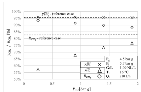
Figure X: Addition of methane recycling loop: influence of intermediate gas pressure
