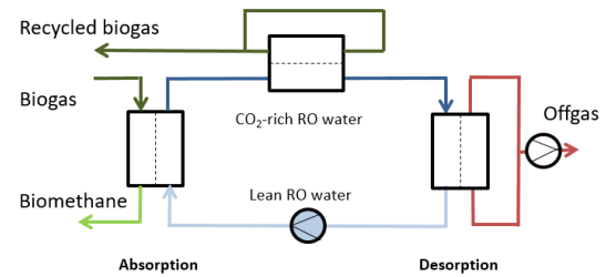
Figure IX: Simplified closed-loop configuration with methane recycling loop
