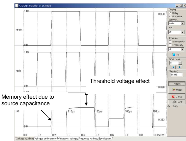
Fig. 15. Typical time-domain waveforms of the gate, drain and source voltages obtained by analog simulation
