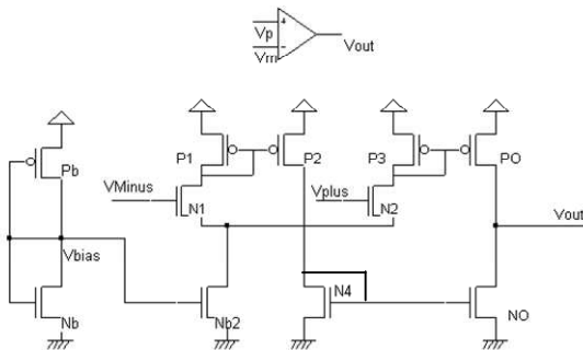
Fig. 19. Schematic diagram of a push-pull operational amplifier
