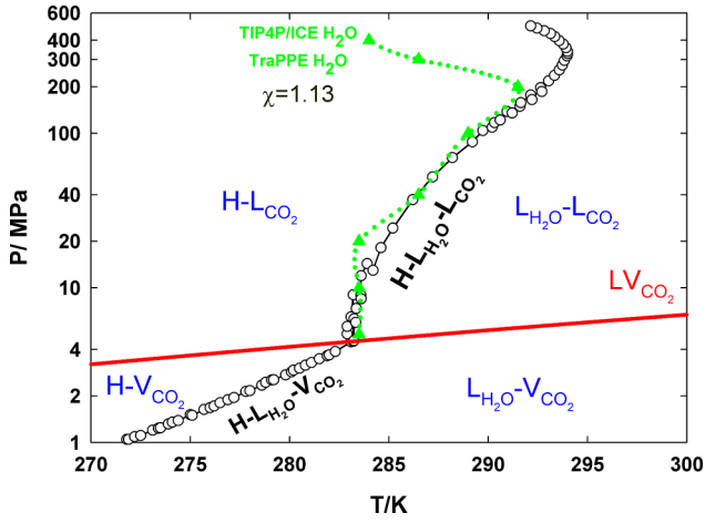
FIG. 10. Estimation of the three-phase coexistence temperature T_3 as a function of pressure for TraPPE \text{CO}_2 in combination with TIP4P/Ice \text{H}_2\text{O} using a positive deviation ( \chi = 1.13 ) of the Lorentz-Berthelot combining rules to model the interaction between \text{CO}_2 and \text{H}_2\text{O} : (green filled triangles) TIP4P/Ice \text{H}_2\text{O} -TraPPE \text{CO}_2 ( \chi = 1.13 ), (black open circles) experimental data, and (red line) experimental \text{CO}_2 vapour pressure curve. Error bars, of the same size as those of Figure 7, have been omitted for clarity.
