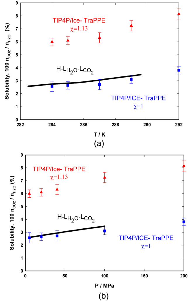
FIG. 11. (a) T-x and (b) P-x projections of the estimated \text{CO}_2 solubility values in \text{H}_2\text{O} , along the three phase line. Solid line represents the experimental correlation by Diamond and Akinfiev, 84 and the symbols are MS results using TIP4P-Ice \text{H}_2\text{O} and TraPPE \text{CO}_2 , using Lorentz Berthelot rules with \chi = 1 (blue squares) and \chi = 1.13 (red triangles).
