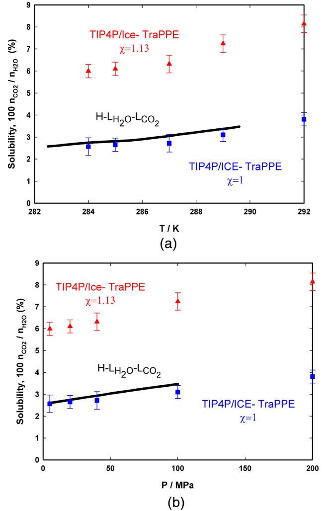
FIG. 11. (a) T - x and (b) P - x projections of the estimated \text{CO}_2 solubility values in \text{H}_2\text{O} , along the three phase line. Solid line represents the experimental correlation by Diamond and Akinfiev, 84 and the symbols are MS results using TIP4P-Ice \text{H}_2\text{O} and TraPPE \text{CO}_2 , using Lorentz Berthelot rules with \chi = 1 (blue squares) and \chi = 1.13 (red triangles).
