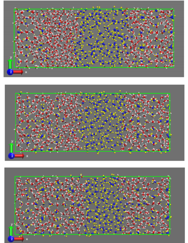
FIG. 6. Snapshots of layer by layer \text{CO}_2 hydrate growth, beginning at the interface of liquid \text{H}_2\text{O} -initial hydrate slab and eventually reaching the hydrate-liquid \text{CO}_2 equilibrium.
