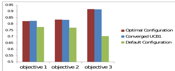
Fig. 5: Average Rewards
