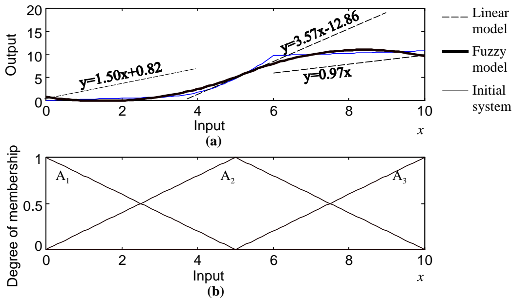
Figure 1 Identifying a Sugeno fuzzy model with given membership functions in the antecedents: (a) the given system, the linear models and the fuzzy model; (b) input membership functions.
