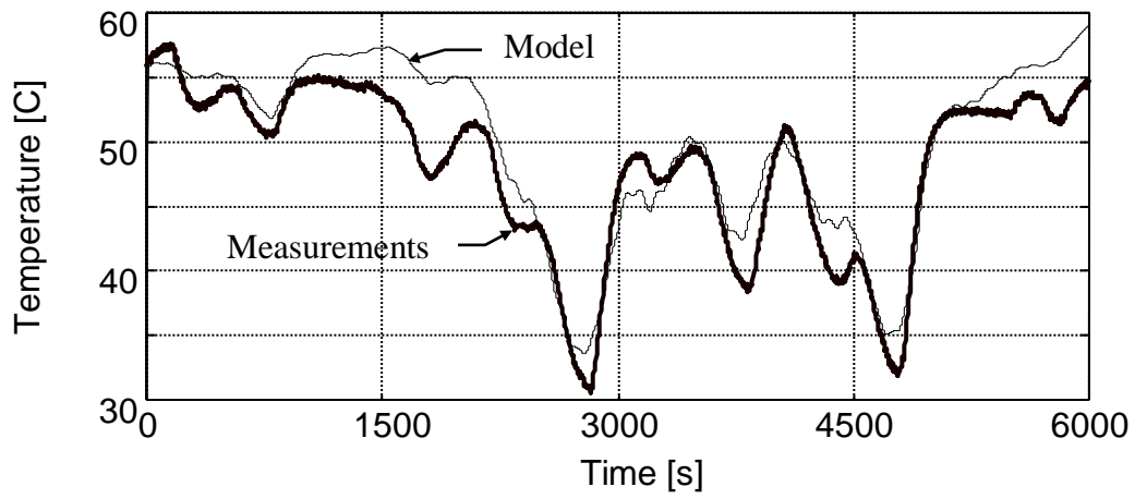
Figure 4 Comparison between the output of the fan-coil and of the model working in recursive prediction. In recursive prediction the model evolves in the next state from a state previously calculated (not measured).
