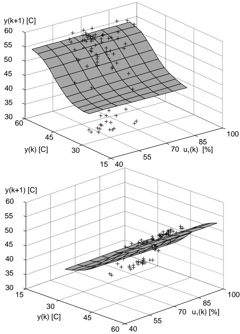
Figure 5 The surface of the identified fuzzy model (considering only the valve position as an input) and the experimentally measured points seen from two angles. The measured points are distributed in space around the surface. The dispersion of the measured points is due to the inputs not considered in the model.
