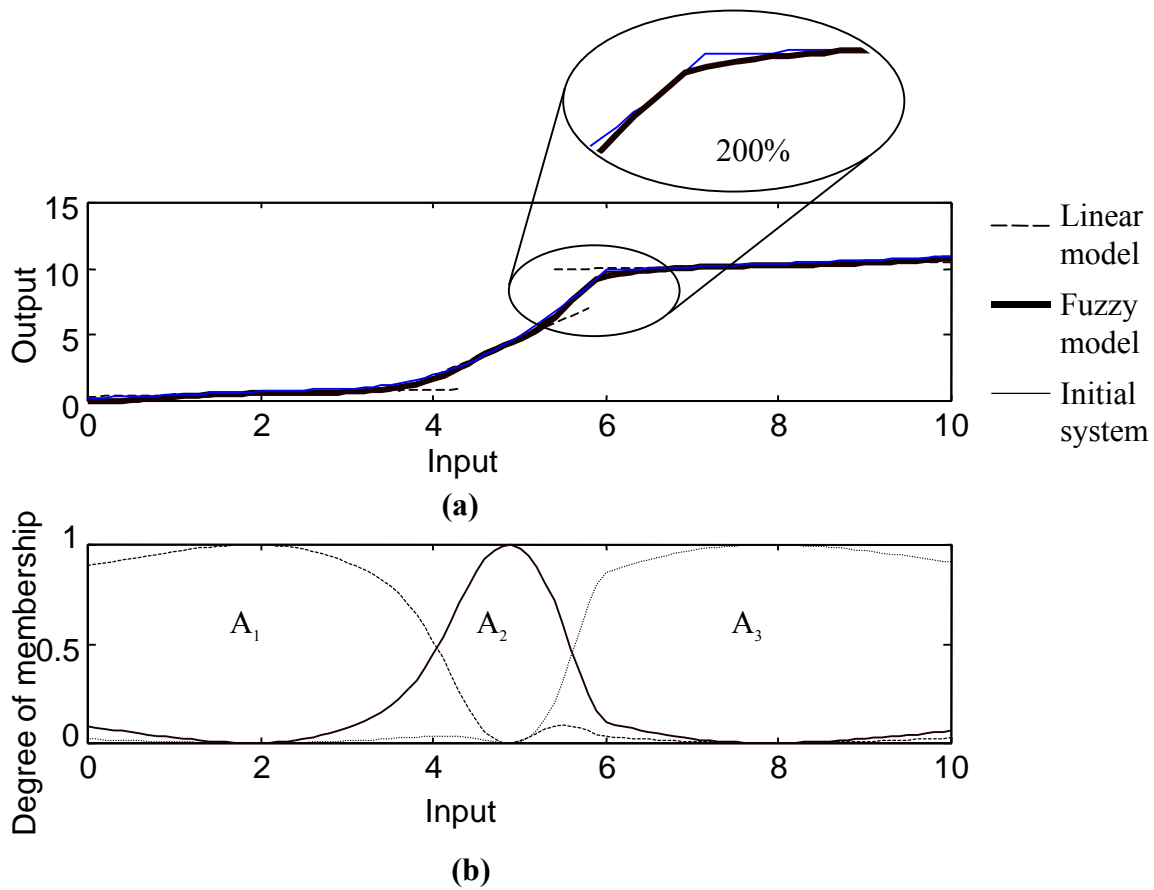
Figure 2 Identifying a Sugeno-type fuzzy model using membership functions determined by Fuzzy C-Means Clustering algorithm. The fuzzy model is better than in Figure 1. (a) The given system, the linear models and the fuzzy model. The fuzzy model is superimposed on the initial system. (b) Input membership functions.
