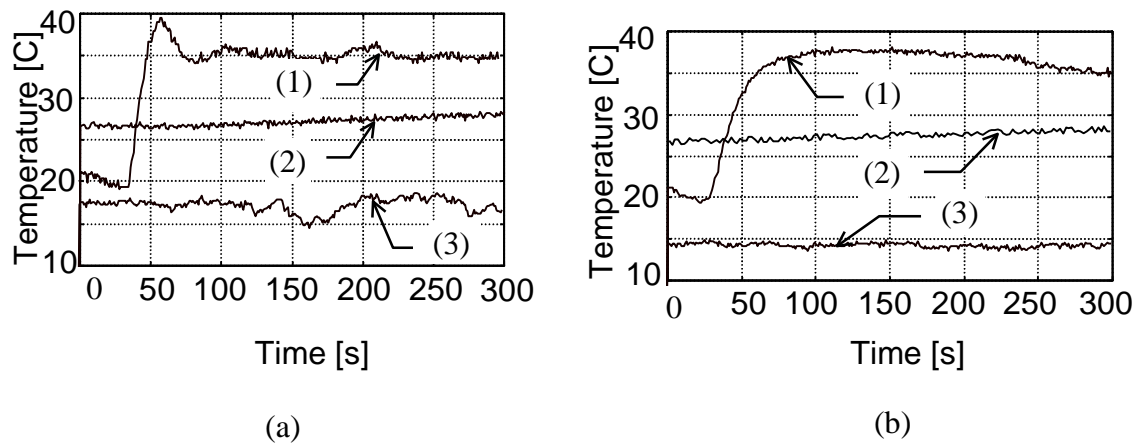
Figure 6 The controlled outlet temperature of a fan-coil when the set point is changed from 20°C to 35°C: a) Sugeno-fuzzy controller; b) PID with anti-wind up. The three temperatures represent: (1) the fan-coil outlet temperature; (2) the indoor air temperature of the test cell; (3) the outdoor air temperature.
