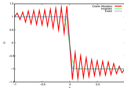
FIG. 1. Burgers equation. Exact solution, implicit Crank-Nicolson scheme, and explicit invariant scheme. Over the spatial domain \Omega = ] - 1, 1[ at time t = 2 . Mesh parameters are set to \Delta x = \Delta t = 5.10^{-2} , and the viscosity is \nu = 75.10^{-5} .
