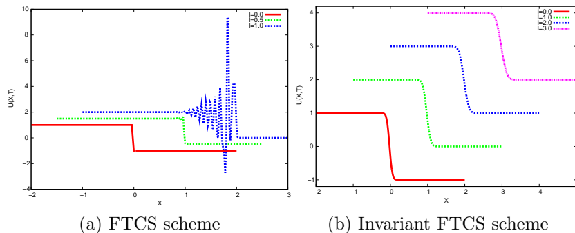
FIG. 2. Burgers equation. Behaviour of numerical solution of (a) : the FTCS scheme, (b) : the IFTCS scheme, for different galilean boost \lambda . Space step size \Delta x is 2.10^{-2} . Viscosity \nu is 5.10^{-3} . CFL is conserved at 1/2 . Time t = 2 .
