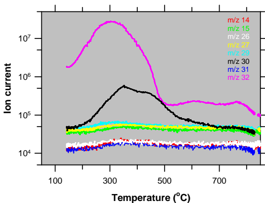
Figure 3. Selected signals versus temperature from CB6 as measured by SAM.
