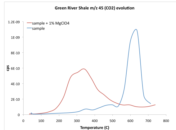
Figure 2. CO 2 evolution from Green River Shale in the presence (red) and absence (blue) of 1% Mg perchlorate.
