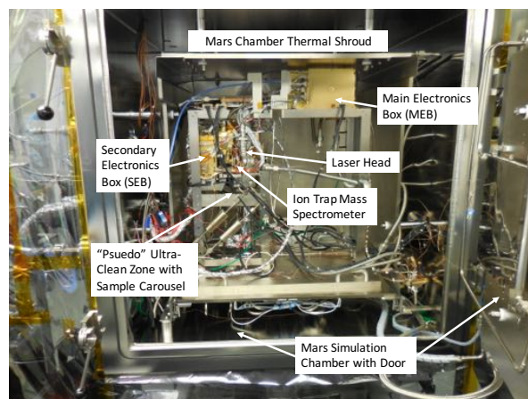
Fig. 1 Flight linear ion trap MS assembly with laser in Mars environment simulation chamber to match mechanical, thermal, pressure, and contamination level that MOMA will experience on the ExoMars rover. Configuration supports either external commercial GC, via gas feedthroughs, or flight model GC within the existing mechanical structure.
